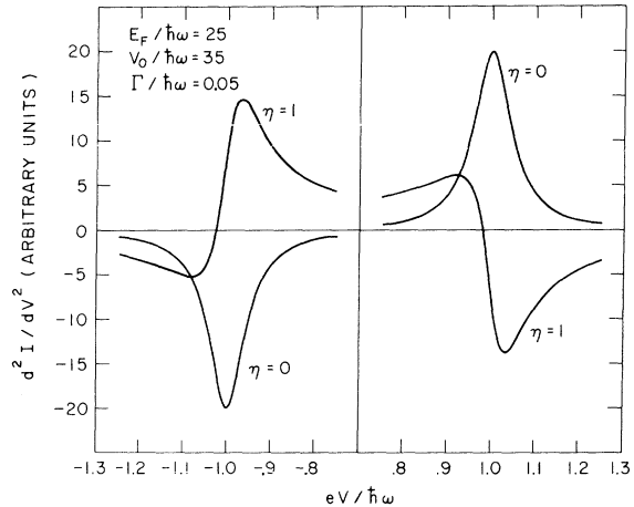
FIG. 3. Curves of d^2I/dV^2 versus V are shown for a typical parameter of a metal-insulator-metal junction. (The background conductance is omitted.) \eta = 0 corresponds to a vibrator far enough inside the tunnel barrier (i. e., more than \sim \frac{1}{2} K) for only the inelastic conductance G_1(V) to be important. \eta = 1 corresponds to a vibrator whose interaction potential is confined to a region near the x=b boundary of the barrier. \Gamma is a parameter representing the finite width of the spectral line of the vibrator. The relative size of the \eta = 1 compared to \eta = 0 line shape depends upon screening and other details of the potential and no attempt has been made to estimate these effects.
